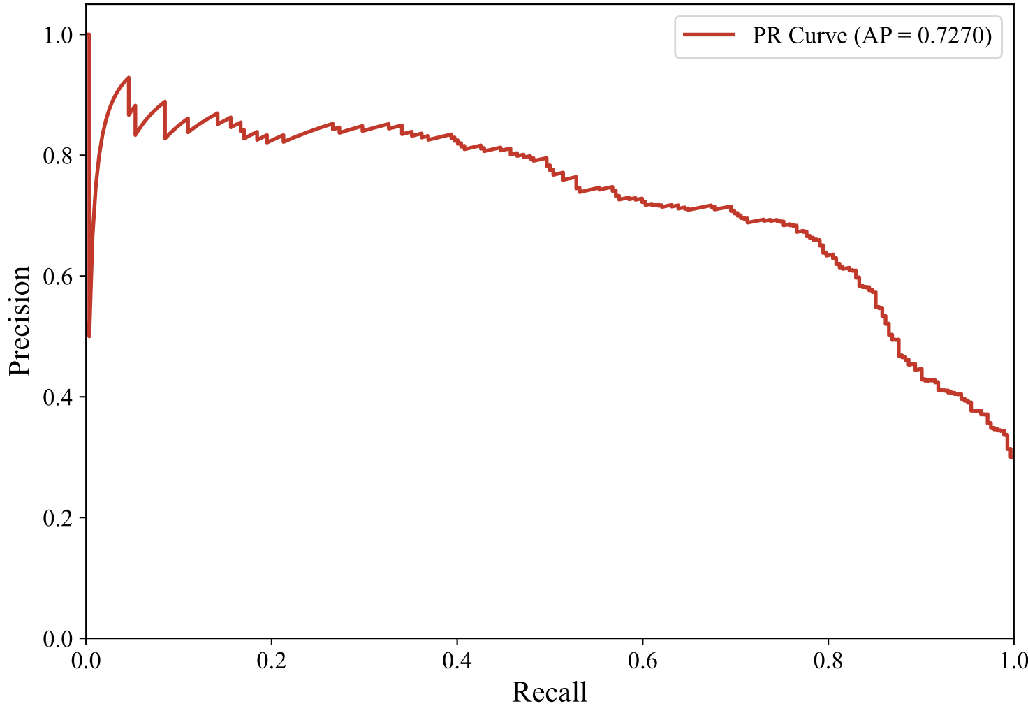
Precision-Recall Curve — ENGLISH_MANUAL (upskyy/bge-m3-korean, LightGBM_Optimized)
