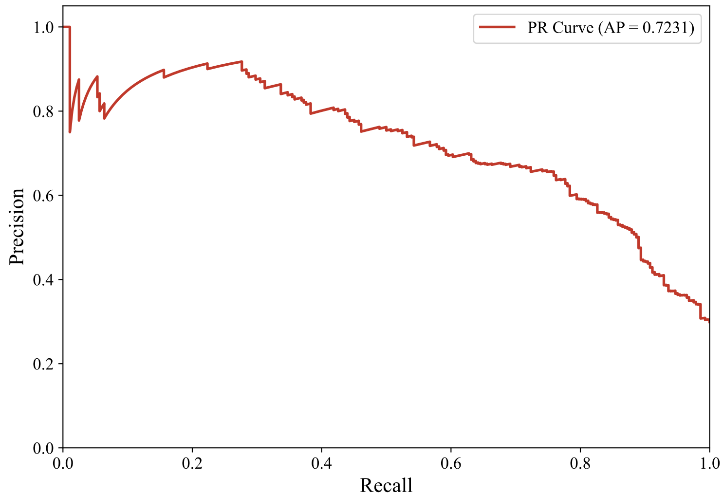
Precision-Recall Curve — ENGLISH_MANUAL (xlm-roberta-base, LightGBM)
