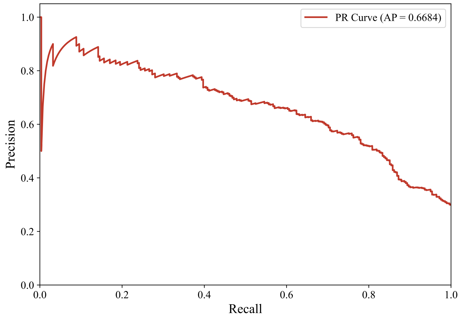
Precision-Recall Curve — ENGLISH_MANUAL (xlm-roberta-base, Random_Forest_Optimized)
