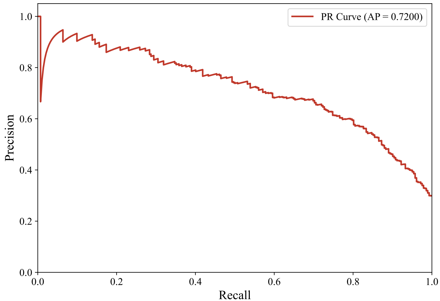
Precision-Recall Curve — ENGLISH_MANUAL (xlm-roberta-base, XGBoost)
