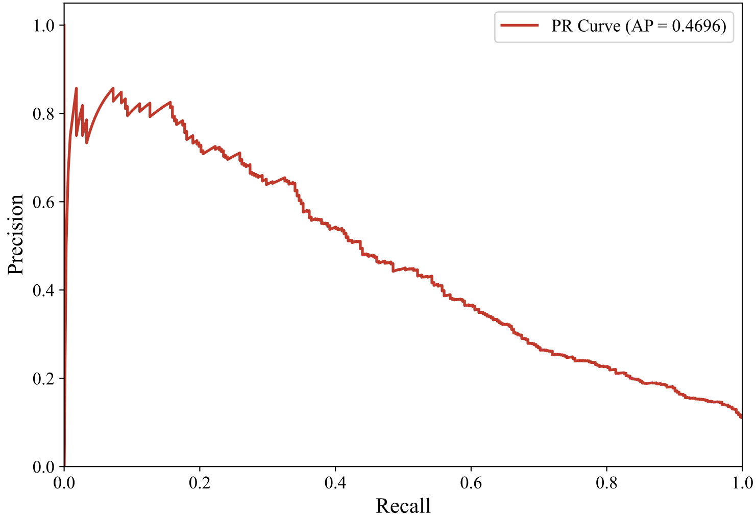
Precision-Recall Curve — GERMAN_MANUAL (bert-base-multilingual-uncased, LightGBM)
