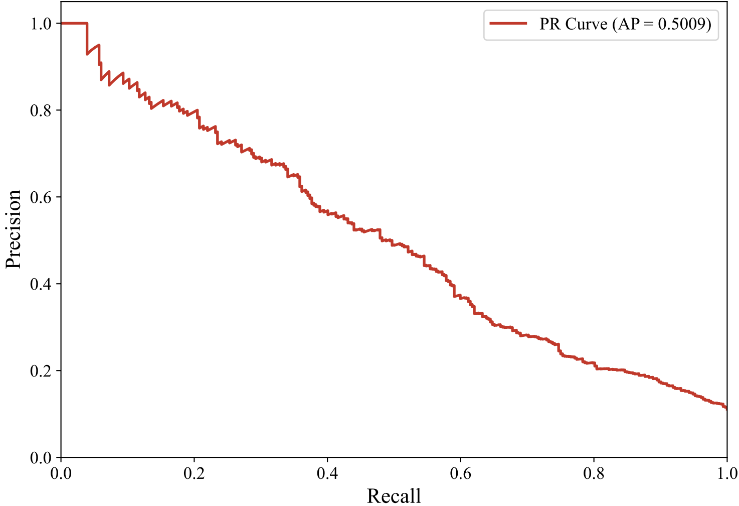
Precision-Recall Curve — GERMAN_MANUAL (efederici/e5-base-multilingual-4096, LightGBM_Optimized)
