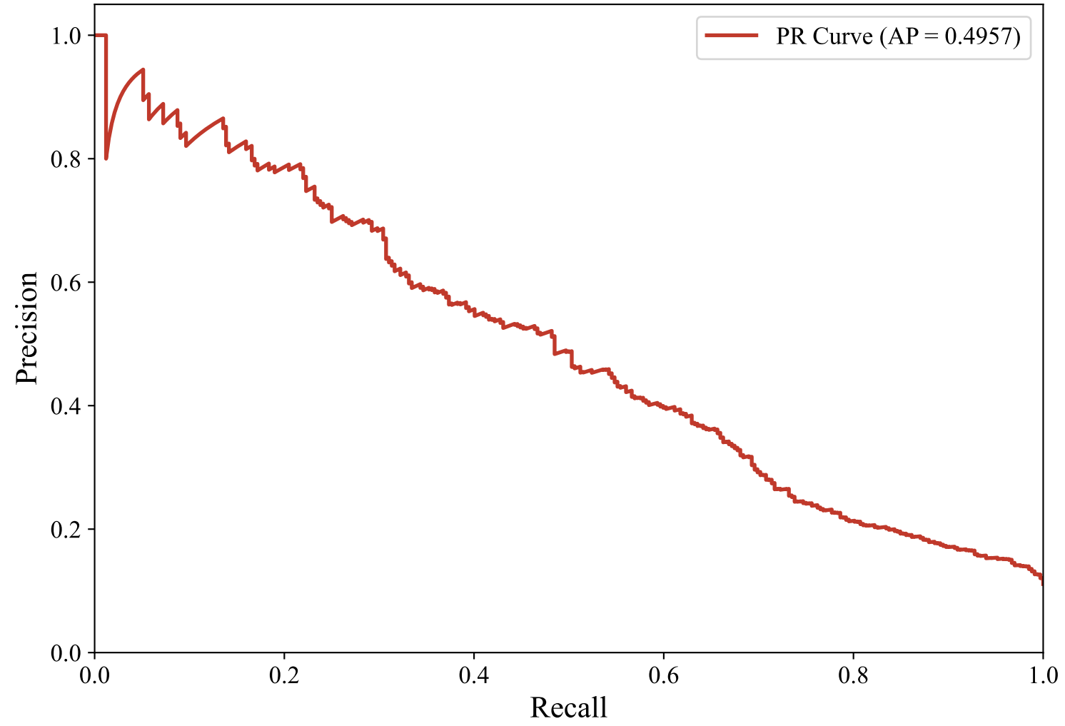
Precision-Recall Curve — GERMAN_MANUAL (efederici/e5-base-multilingual-4096, XGBoost)
