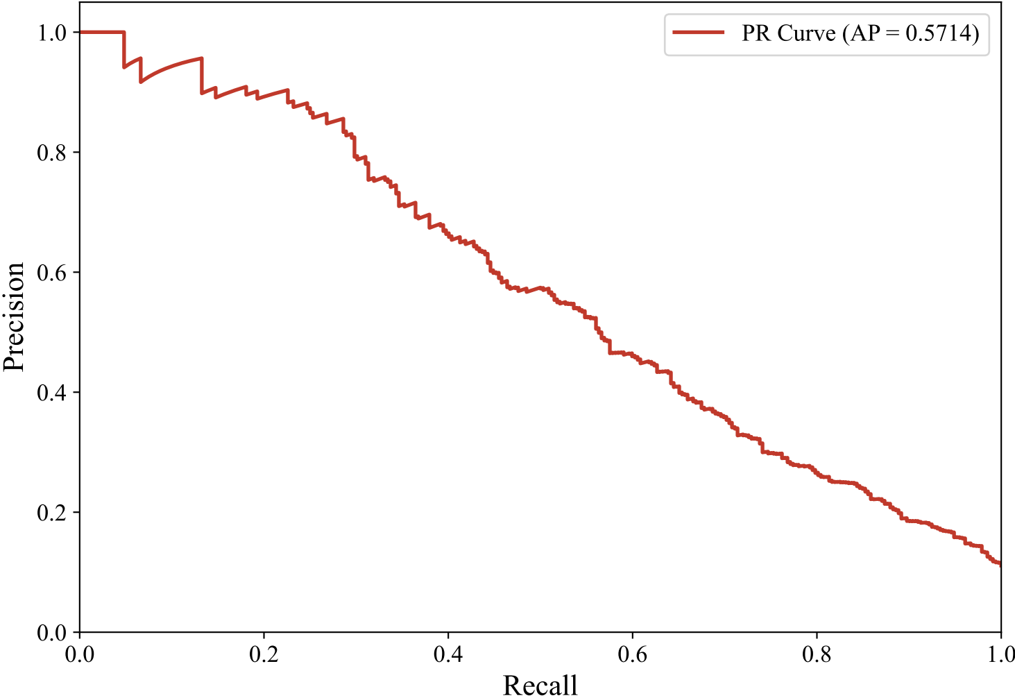
Precision-Recall Curve — GERMAN_MANUAL (intfloat/multilingual-e5-large-instruct, LightGBM_Optimized)
