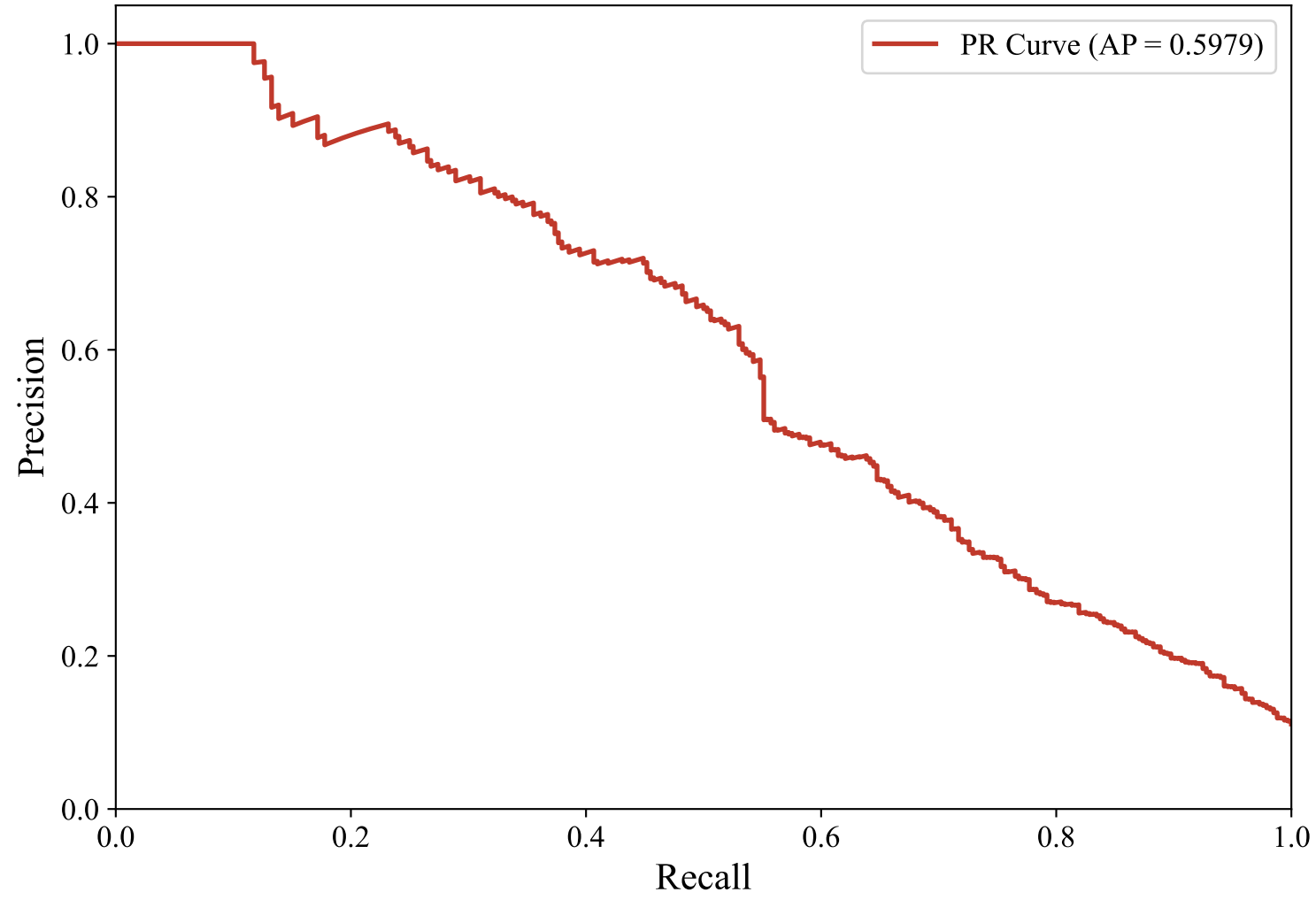
Precision-Recall Curve — GERMAN_MANUAL (intfloat/multilingual-e5-large-instruct, XGBoost)
