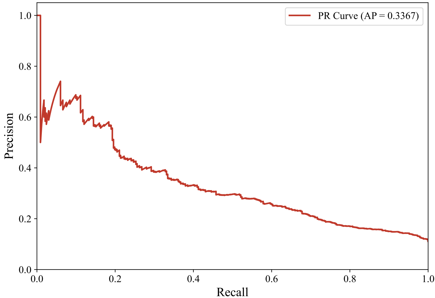
Precision-Recall Curve — GERMAN_MANUAL (paraphrase-multilingual-mpnet-base-v2, Random_Forest)
