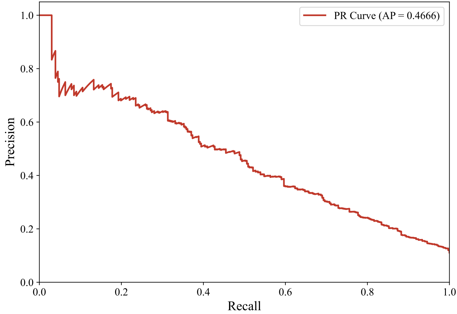
Precision-Recall Curve — GERMAN_MANUAL (snowflake-arctic-embed-l-v2.0, Random_Forest)
