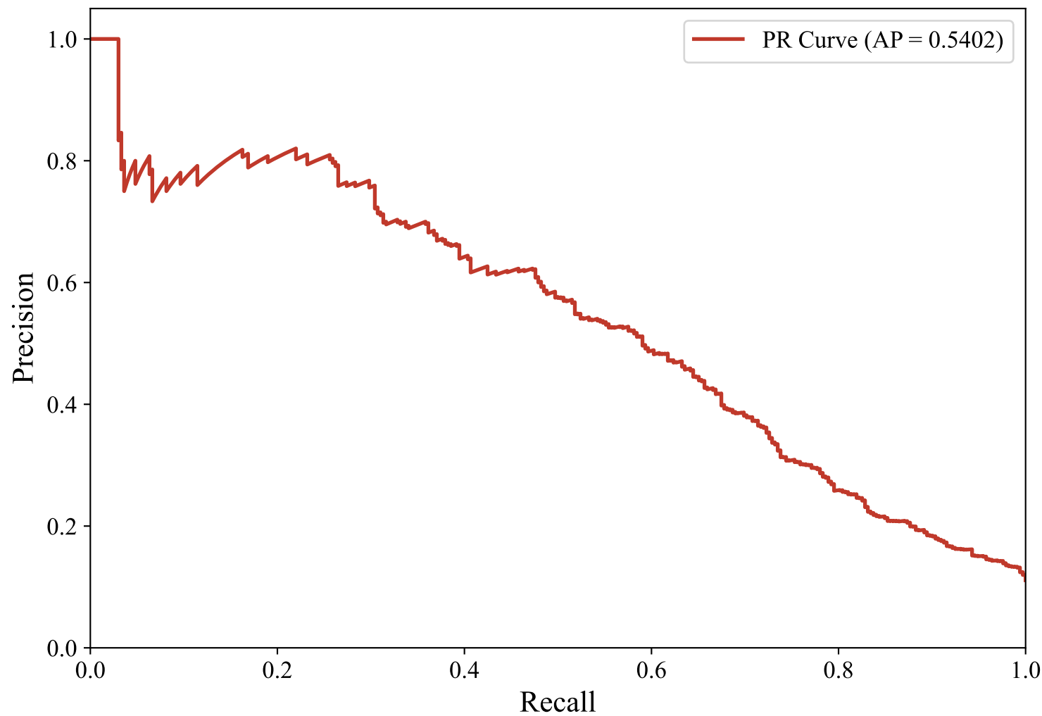
Precision-Recall Curve — GERMAN_MANUAL (snowflake-arctic-embed-l-v2.0, Voting_Ensemble)
