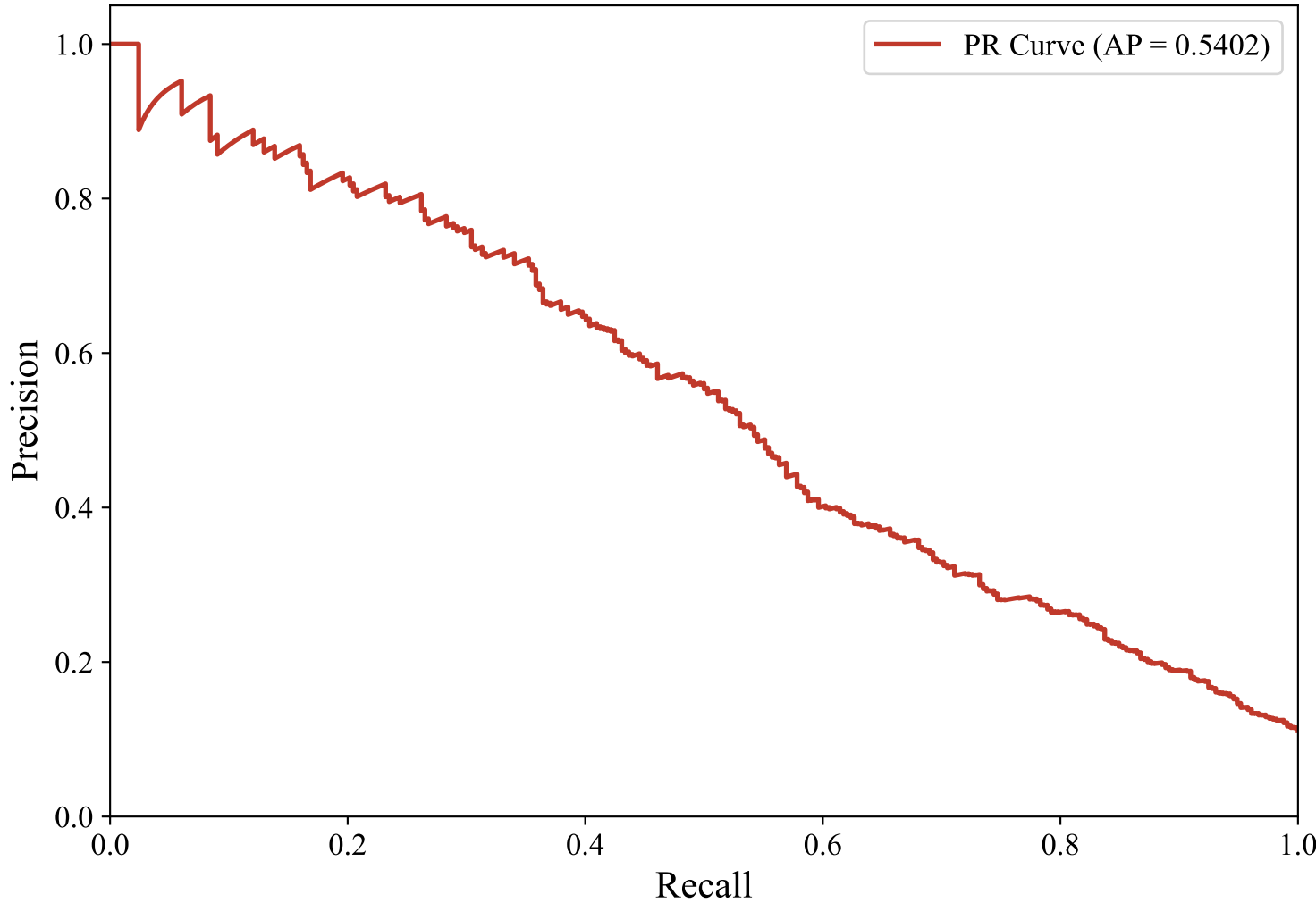
Precision-Recall Curve — GERMAN_MANUAL (upskyy/bge-m3-korean, LightGBM_Optimized)
