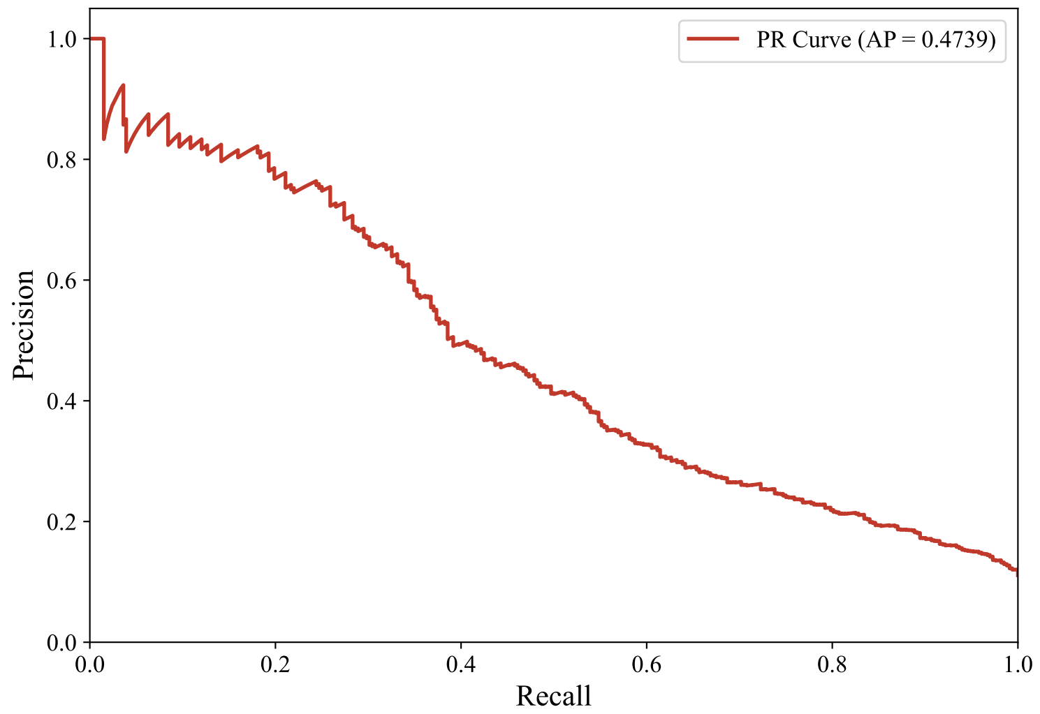
Precision-Recall Curve — GERMAN_MANUAL (upskyy/bge-m3-korean, Random_Forest)
