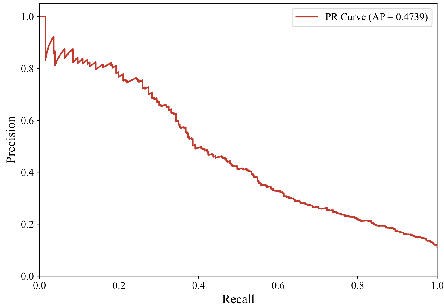
Precision-Recall Curve — GERMAN_MANUAL (upskyy/bge-m3-korean, Random_Forest_Optimized)
