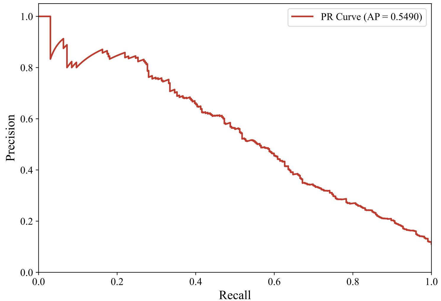
Precision-Recall Curve — GERMAN_MANUAL (upskyy/bge-m3-korean, Voting_Ensemble)
