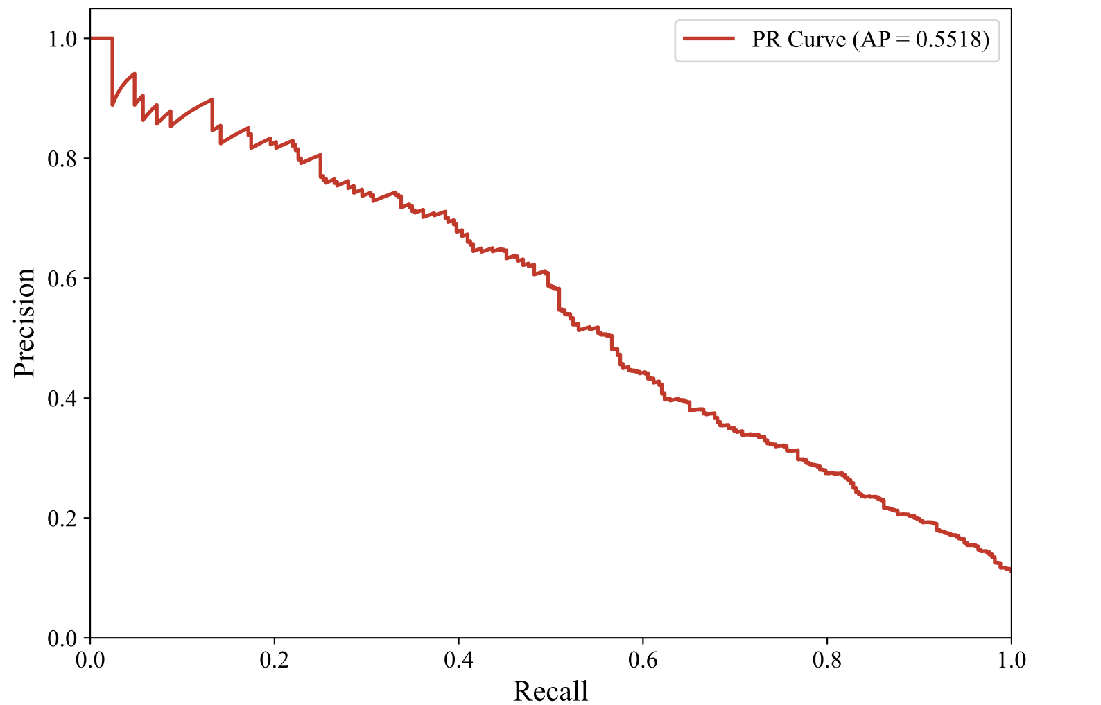
Precision-Recall Curve — GERMAN_MANUAL (upskyy/bge-m3-korean, XGBoost)
