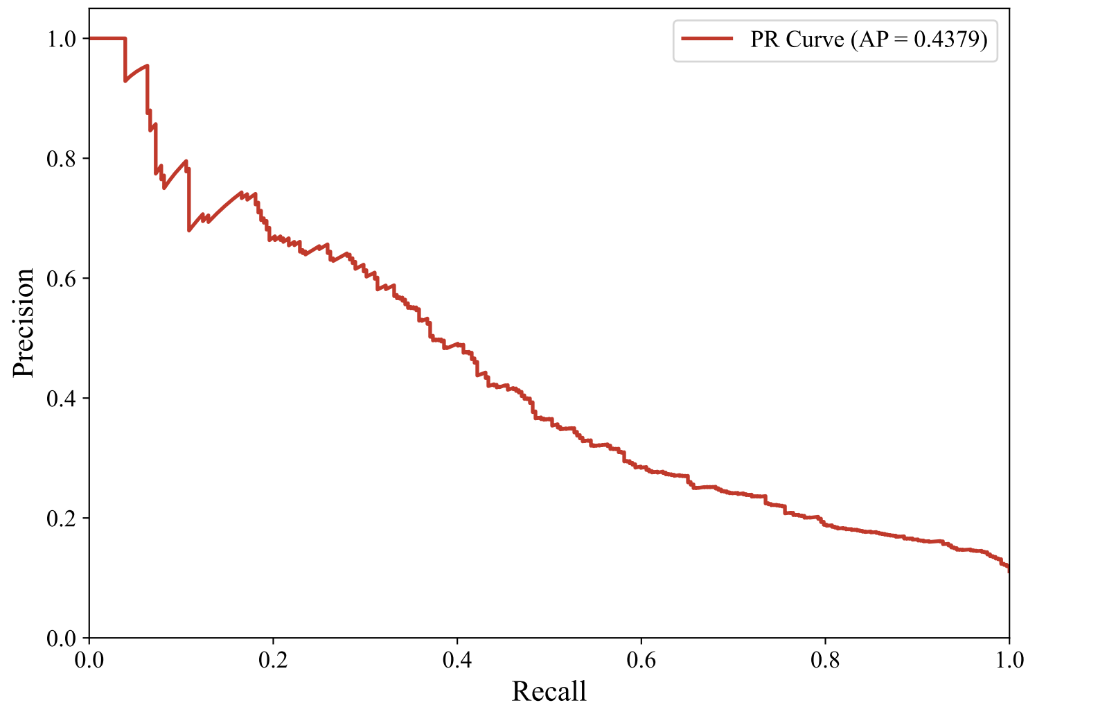
Precision-Recall Curve — GERMAN_MANUAL (xlm-roberta-base, Random_Forest_Optimized)
