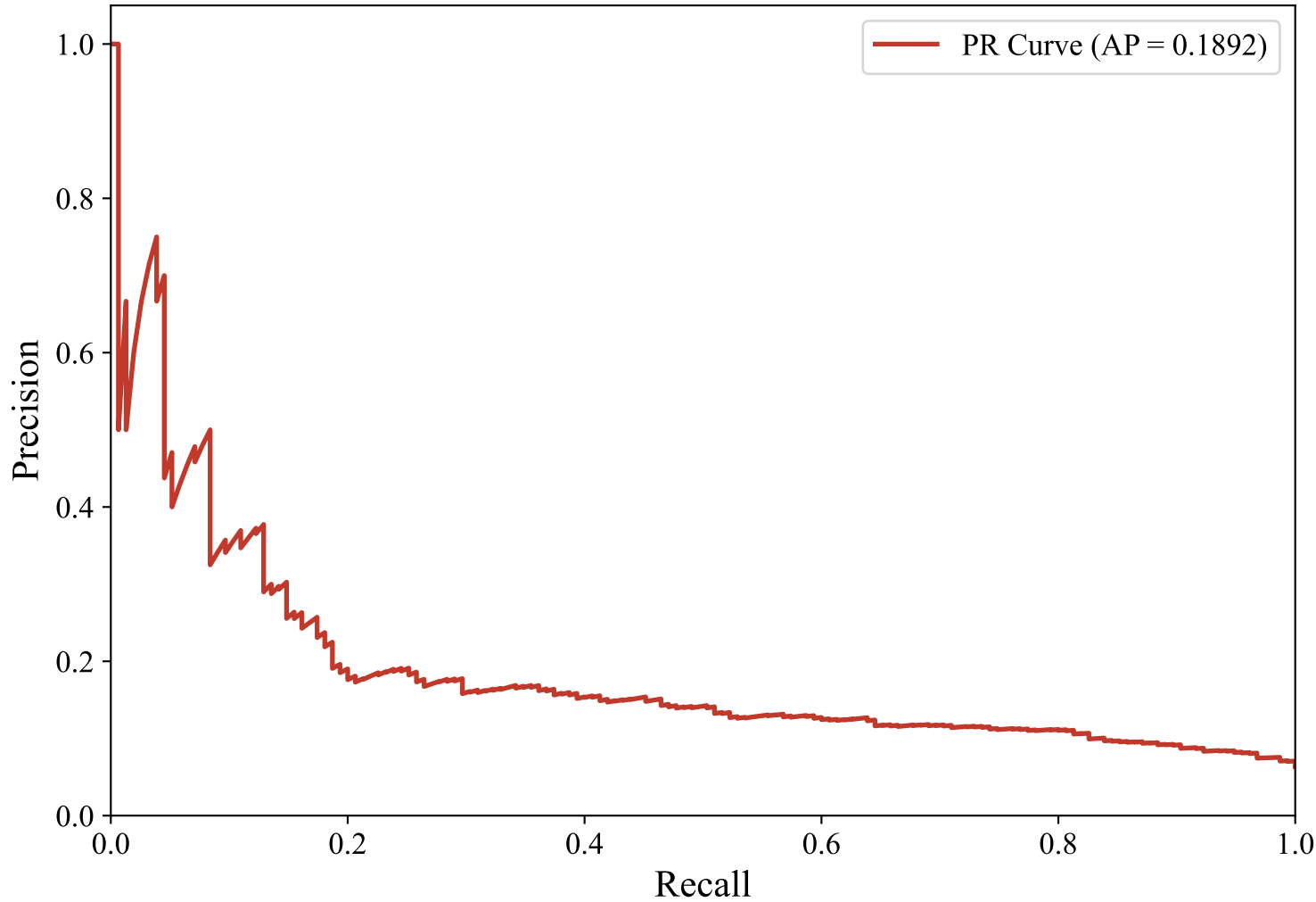
Precision-Recall Curve — SWEDISH_MANUAL (bert-base-multilingual-uncased, LightGBM_Optimized)
