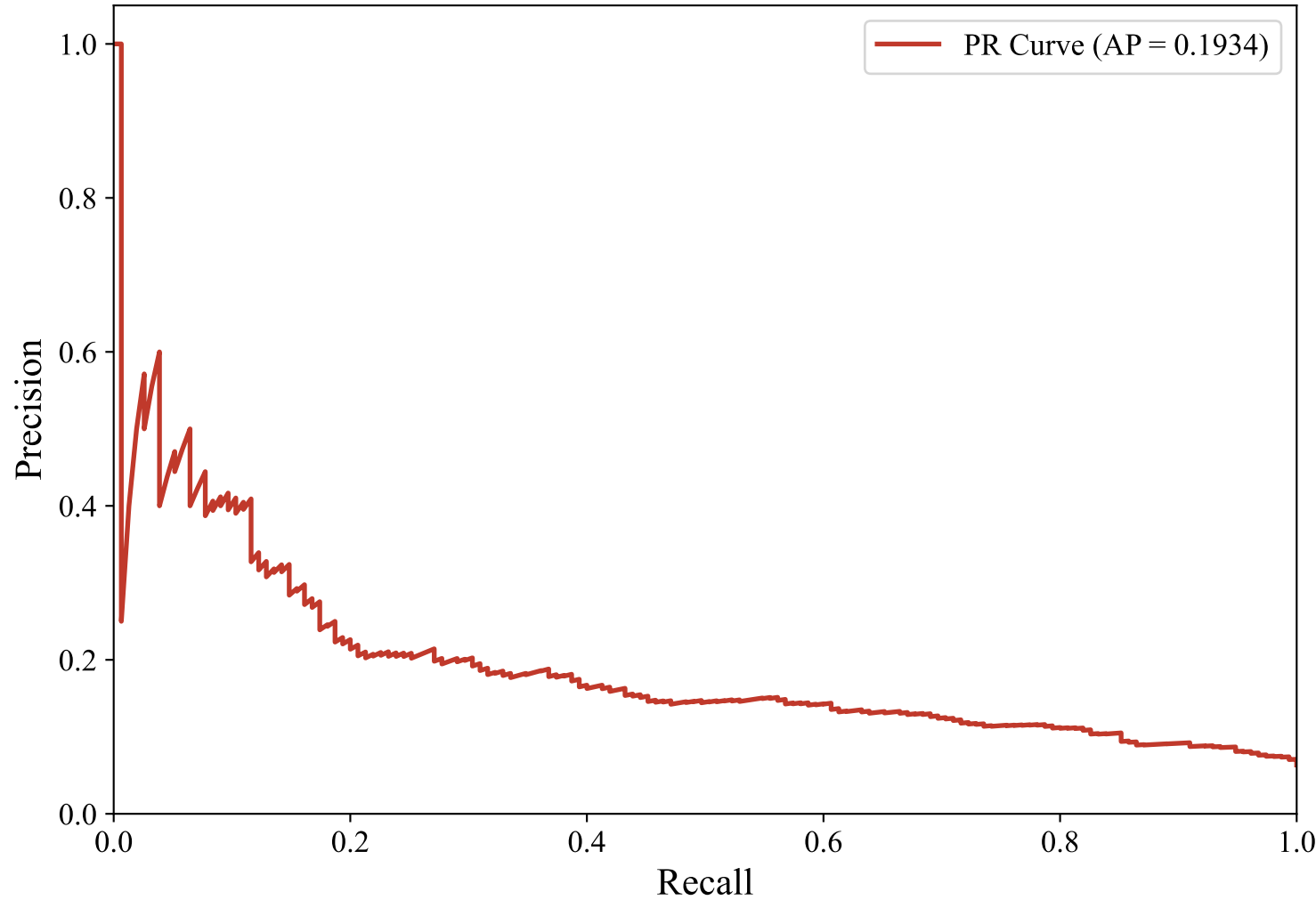
Precision-Recall Curve — SWEDISH_MANUAL (bert-base-multilingual-uncased, Voting_Ensemble)
