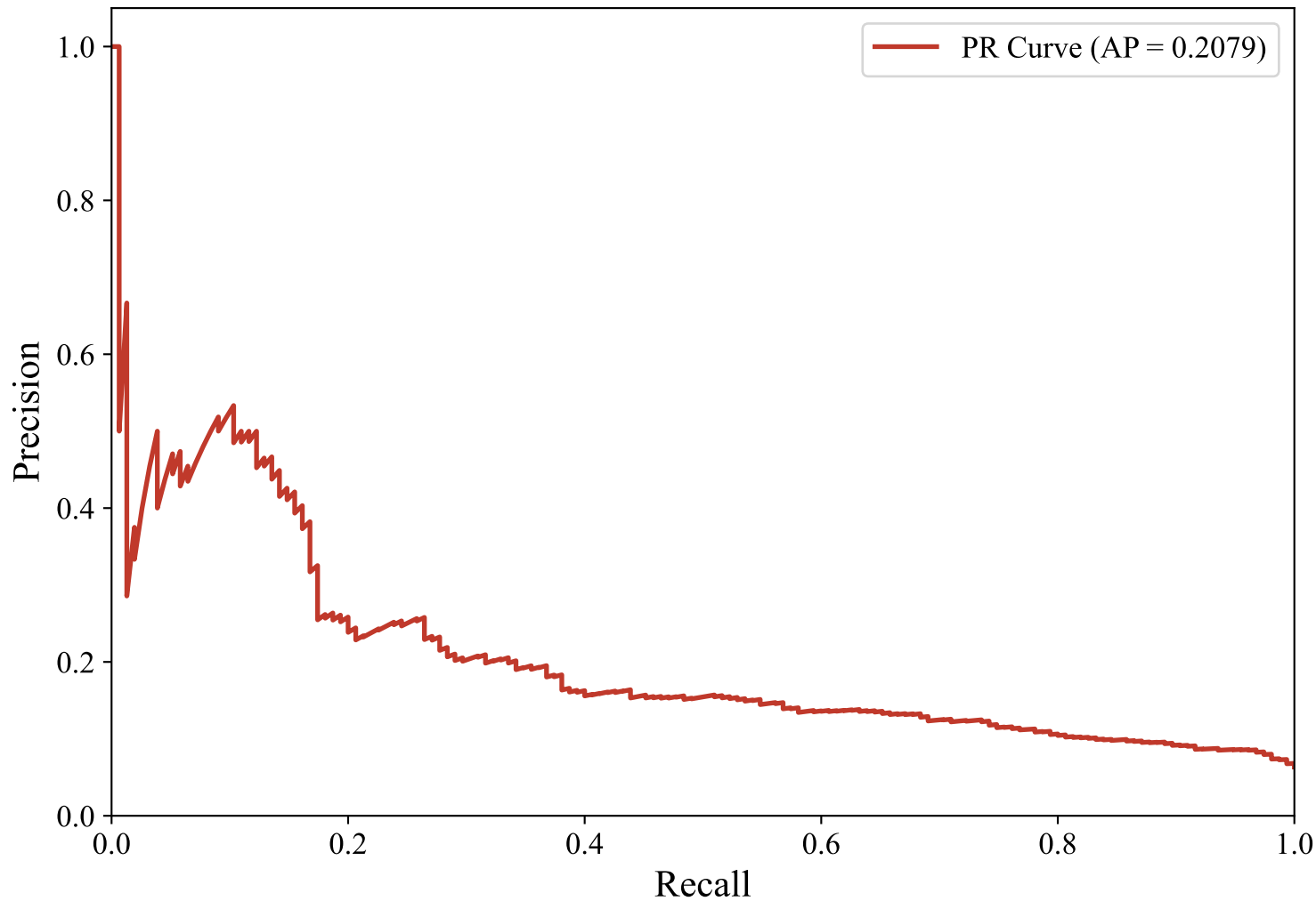
Precision-Recall Curve — SWEDISH_MANUAL (bert-base-multilingual-uncased, XGBoost_Optimized)
