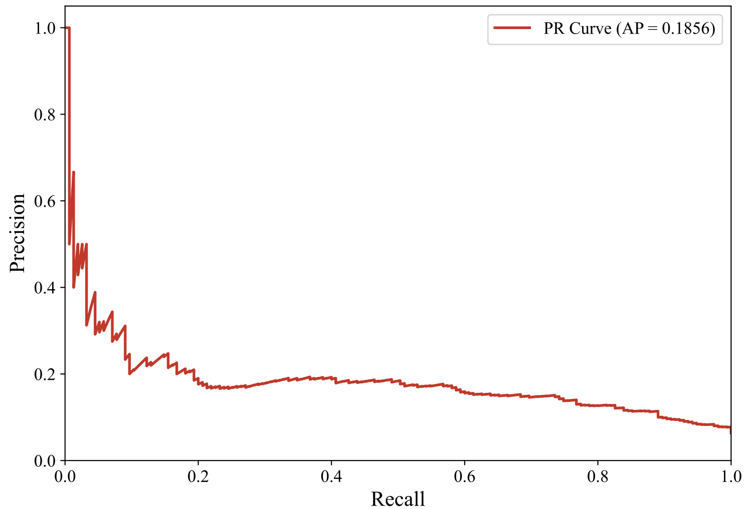
Precision-Recall Curve — SWEDISH_MANUAL (efederici/e5-base-multilingual-4096, Random_Forest_Optimized)
