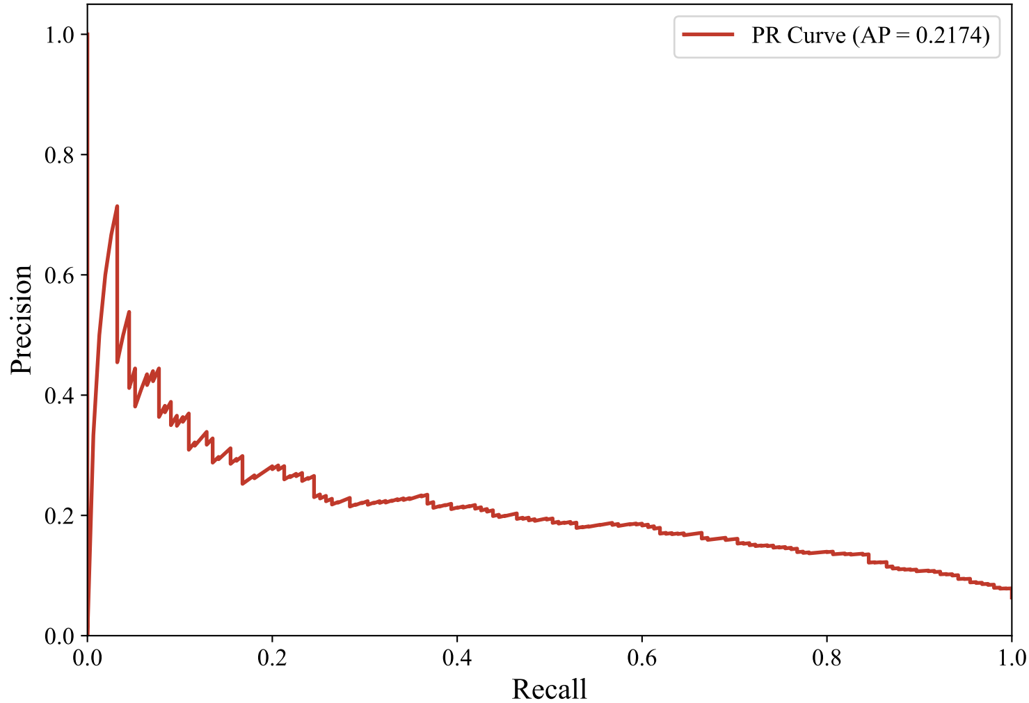
Precision-Recall Curve — SWEDISH_MANUAL (efederici/e5-base-multilingual-4096, Voting_Ensemble)
