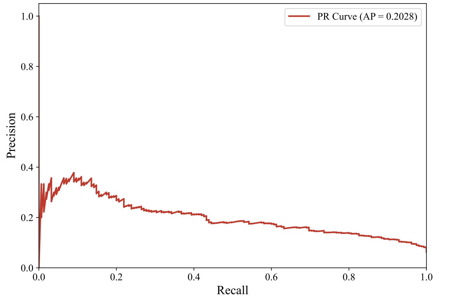
Precision-Recall Curve — SWEDISH_MANUAL (intfloat/multilingual-e5-large-instruct, Random_Forest)
