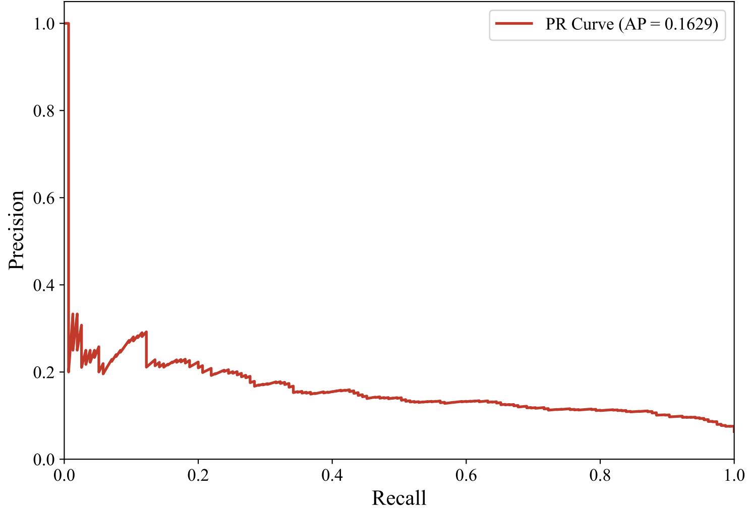
Precision-Recall Curve — SWEDISH_MANUAL (paraphrase-multilingual-MiniLM-L12-v2, Random_Forest_Optimized)
