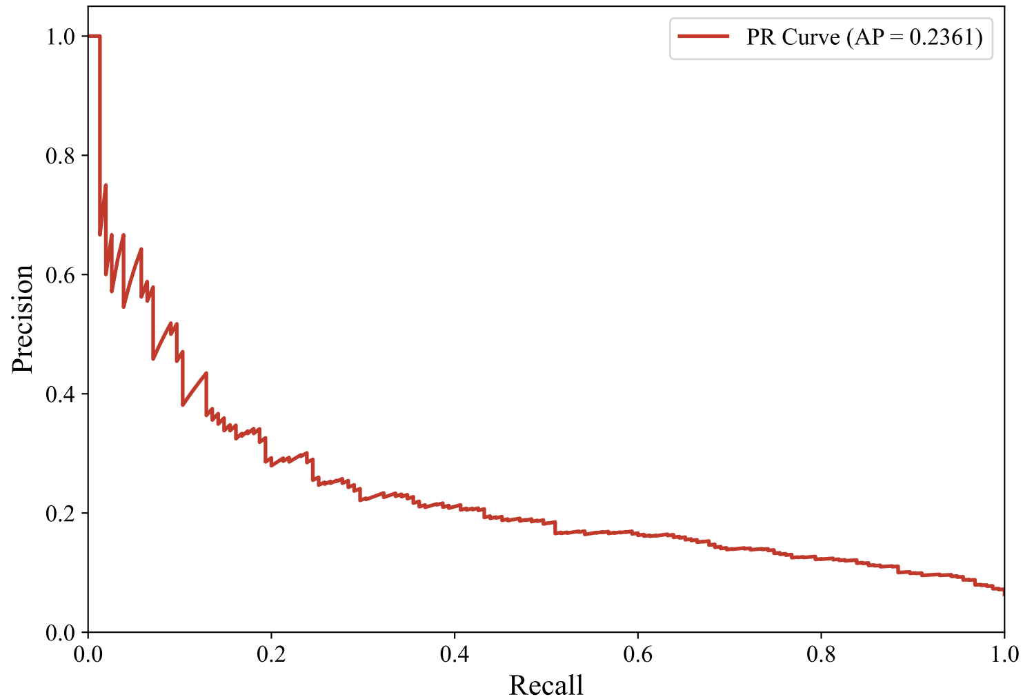
Precision-Recall Curve — SWEDISH_MANUAL (paraphrase-multilingual-mpnet-base-v2, LightGBM_Optimized)
