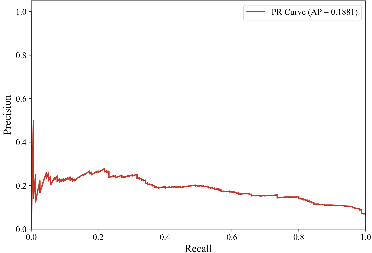
Precision-Recall Curve — SWEDISH_MANUAL (snowflake-arctic-embed-l-v2.0, Random_Forest_Optimized)
