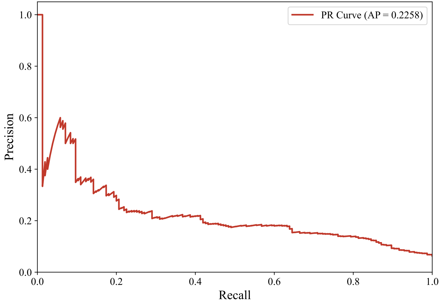
Precision-Recall Curve — SWEDISH_MANUAL (upskyy/bge-m3-korean, LightGBM_Optimized)
