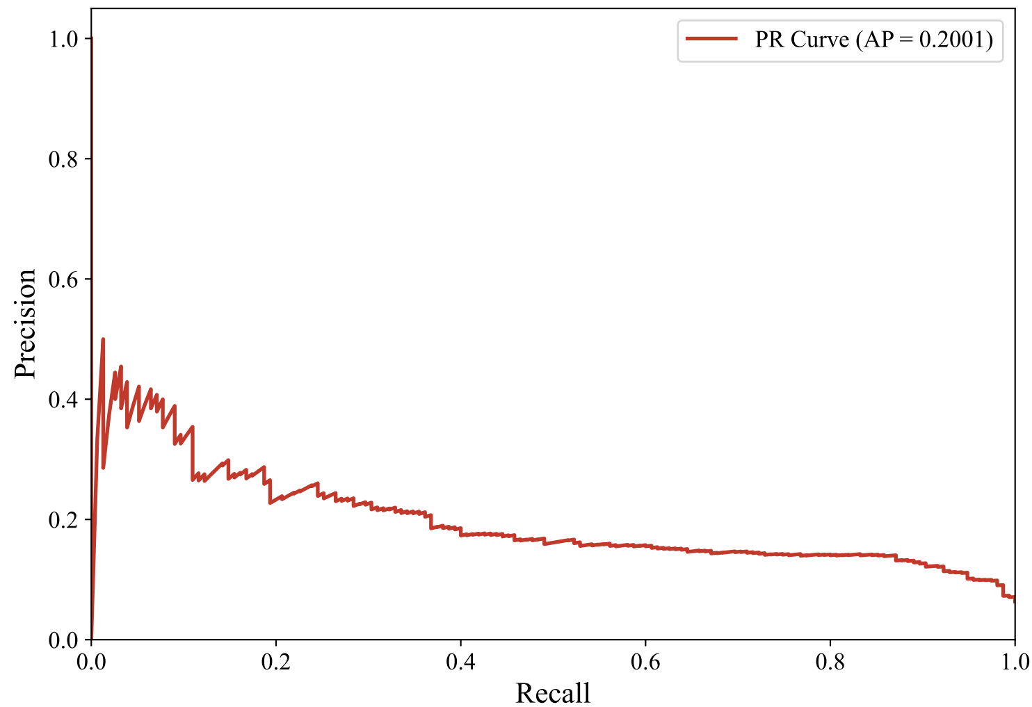
Precision-Recall Curve — SWEDISH_MANUAL (upskyy/bge-m3-korean, Random_Forest)
