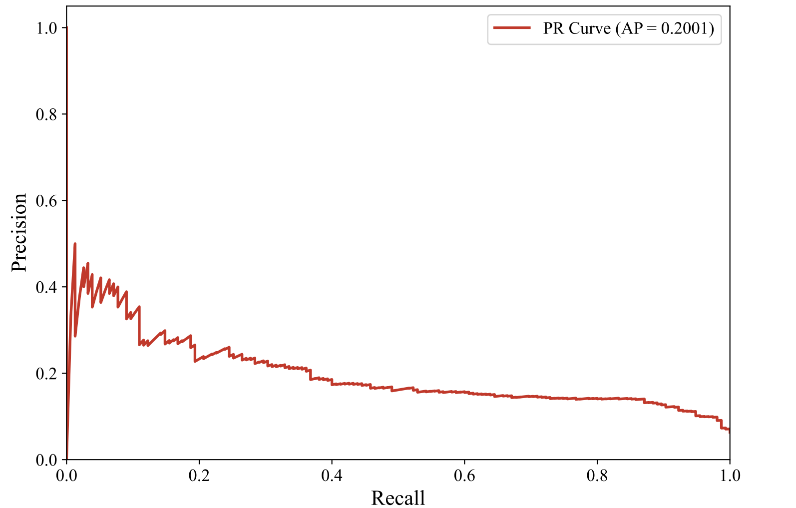
Precision-Recall Curve — SWEDISH_MANUAL (upskyy/bge-m3-korean, Random_Forest_Optimized)
