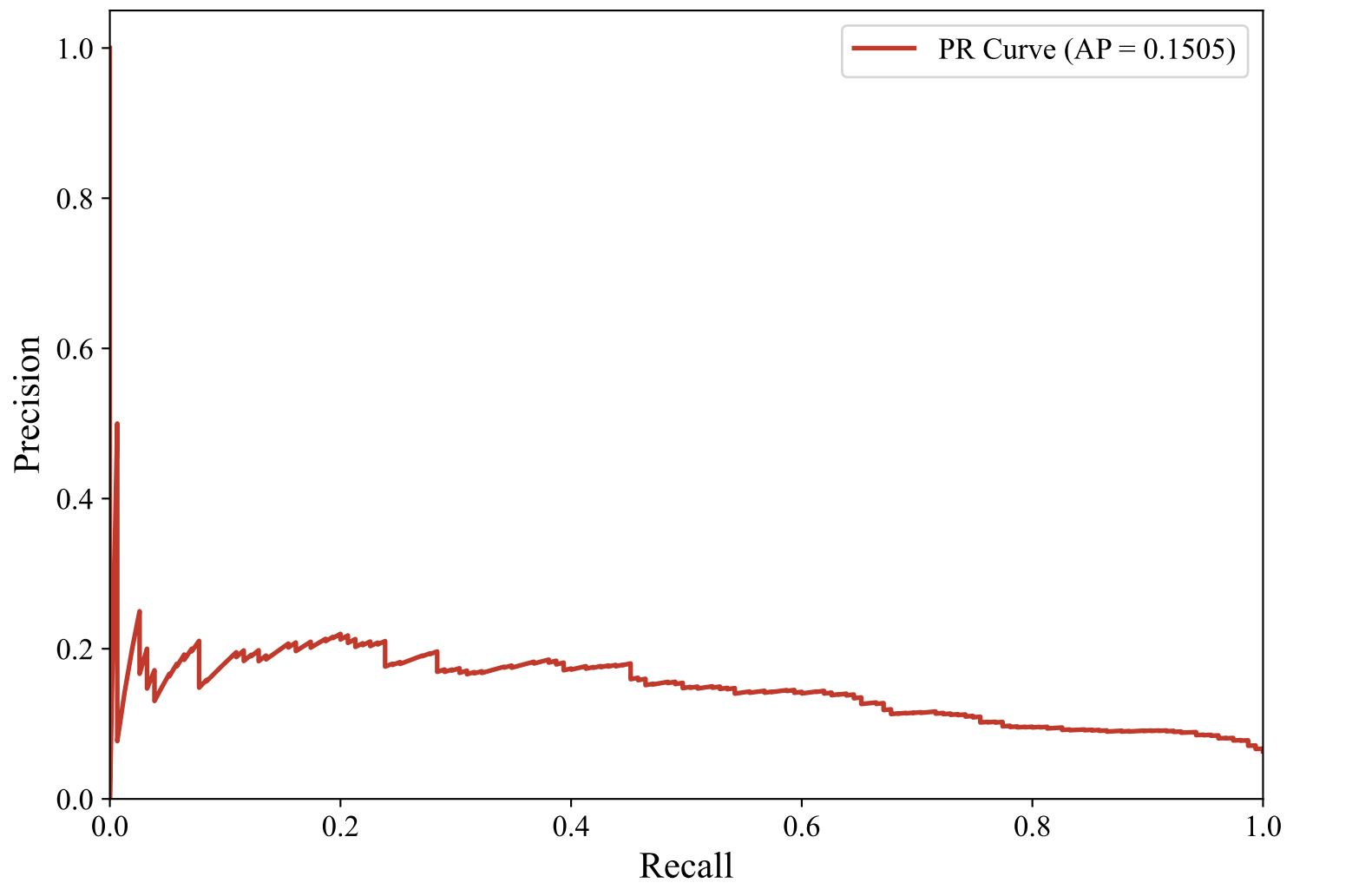
Precision-Recall Curve — SWEDISH_MANUAL (xlm-roberta-base, Random_Forest)
