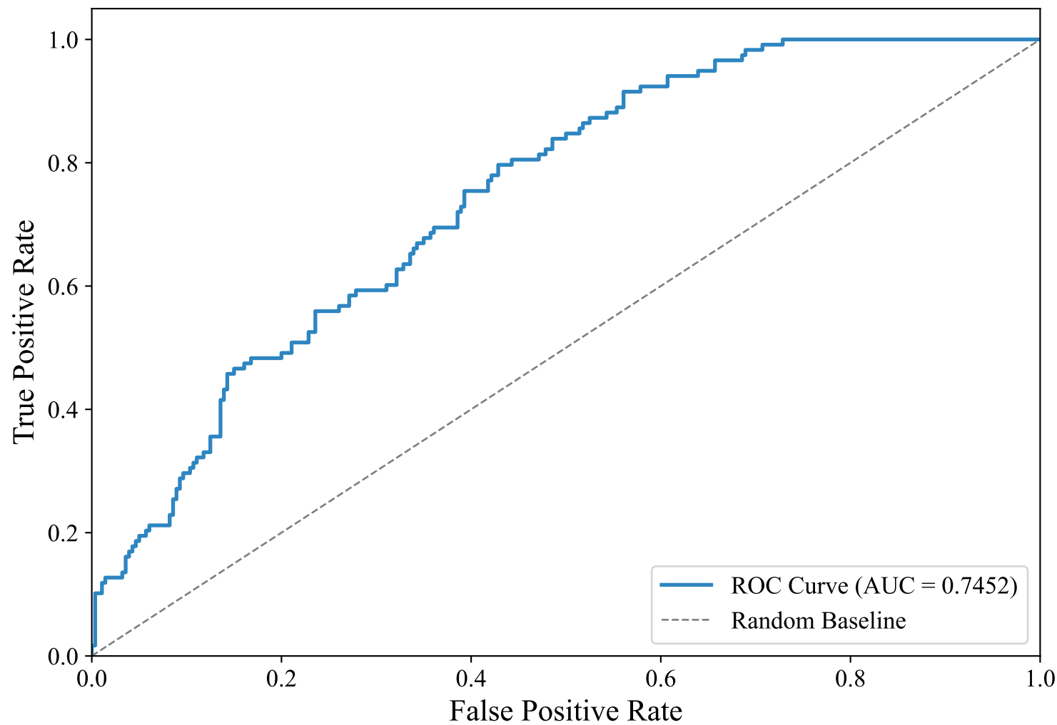
ROC Curve — DUTCH_MANUAL (efederici/e5-base-multilingual-4096, Random_Forest)
