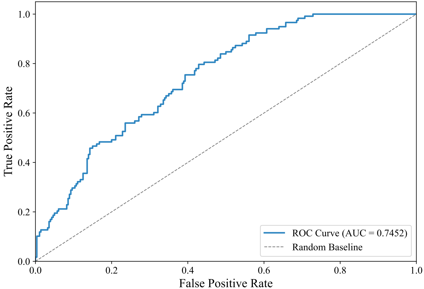
ROC Curve — DUTCH_MANUAL (efederici/e5-base-multilingual-4096, Random_Forest_Optimized)
