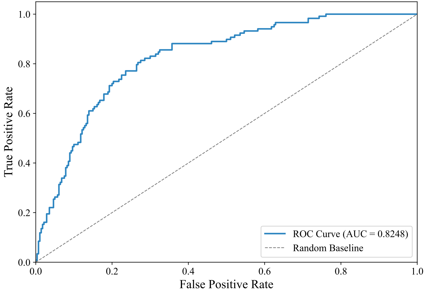
ROC Curve — DUTCH_MANUAL (intfloat/multilingual-e5-large-instruct, LightGBM_Optimized)
