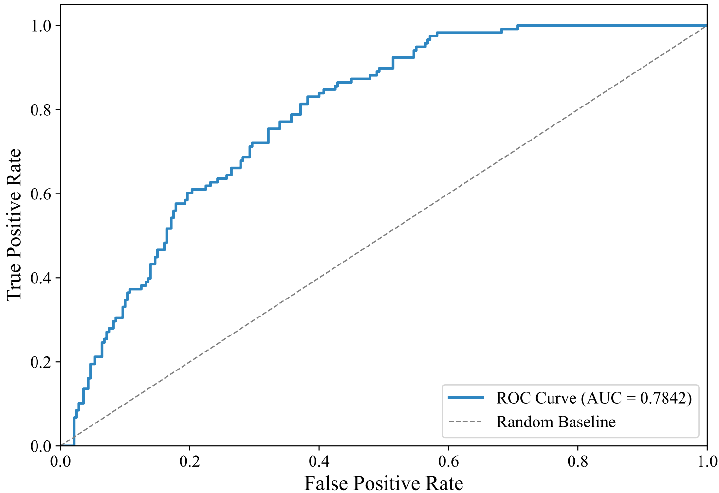
ROC Curve — DUTCH_MANUAL (intfloat/multilingual-e5-large-instruct, Random_Forest_Optimized)
