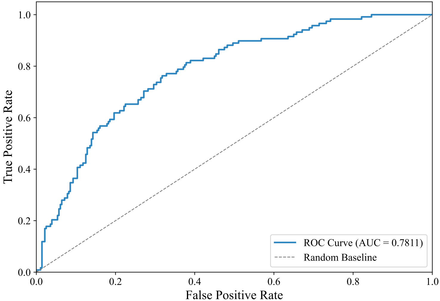
ROC Curve — DUTCH_MANUAL (paraphrase-multilingual-MiniLM-L12-v2, LightGBM)
