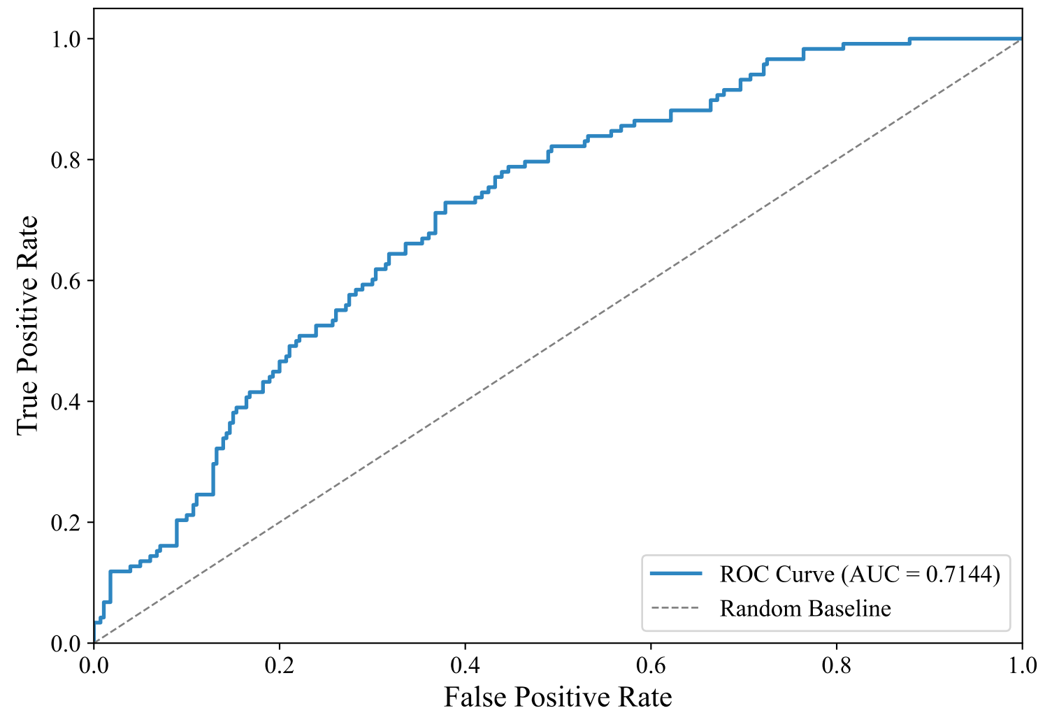
ROC Curve — DUTCH_MANUAL (paraphrase-multilingual-MiniLM-L12-v2, Random_Forest)
