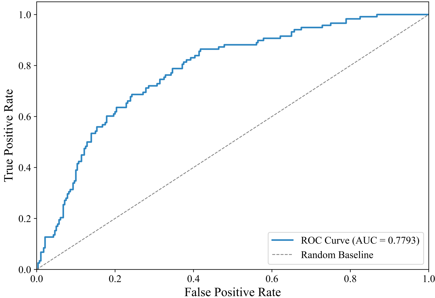
ROC Curve — DUTCH_MANUAL (paraphrase-multilingual-MiniLM-L12-v2, Voting_Ensemble)
