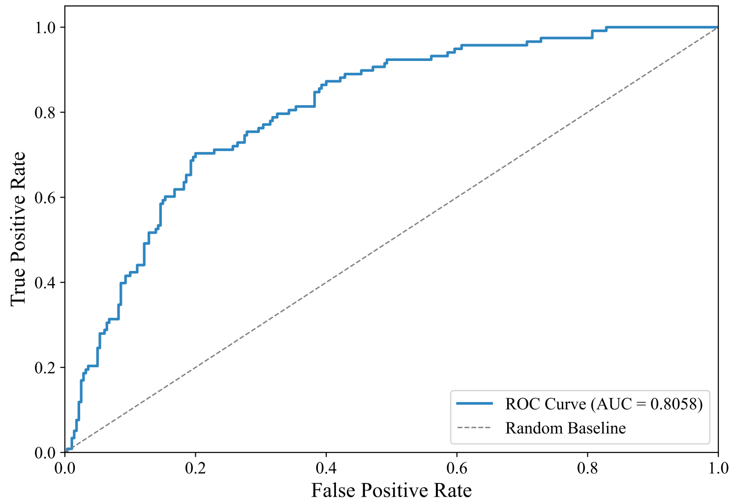
ROC Curve — DUTCH_MANUAL (paraphrase-multilingual-mpnet-base-v2, Voting_Ensemble)
