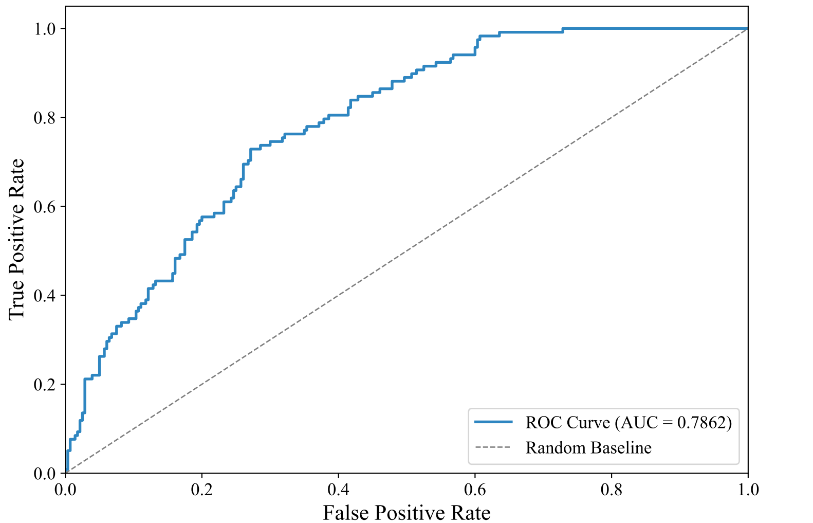
ROC Curve — DUTCH_MANUAL (snowflake-arctic-embed-l-v2.0, Random_Forest_Optimized)
