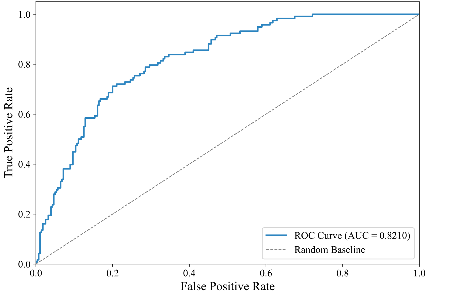
ROC Curve — DUTCH_MANUAL (snowflake-arctic-embed-l-v2.0, XGBoost)
