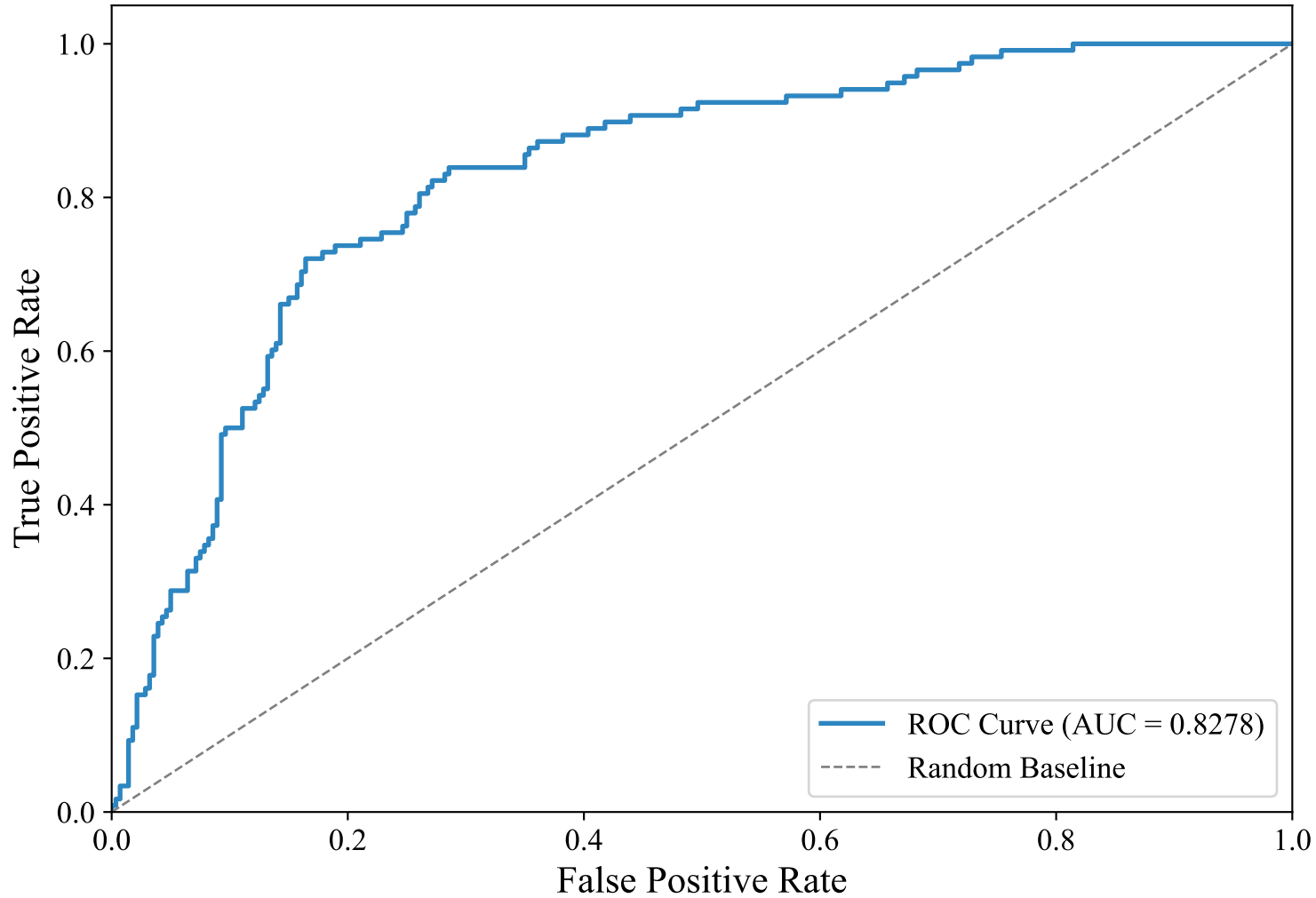
ROC Curve — DUTCH_MANUAL (upskyy/bge-m3-korean, LightGBM_Optimized)
