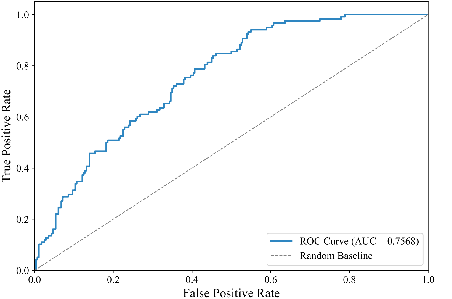
ROC Curve — DUTCH_MANUAL (xlm-roberta-base, Random_Forest)
