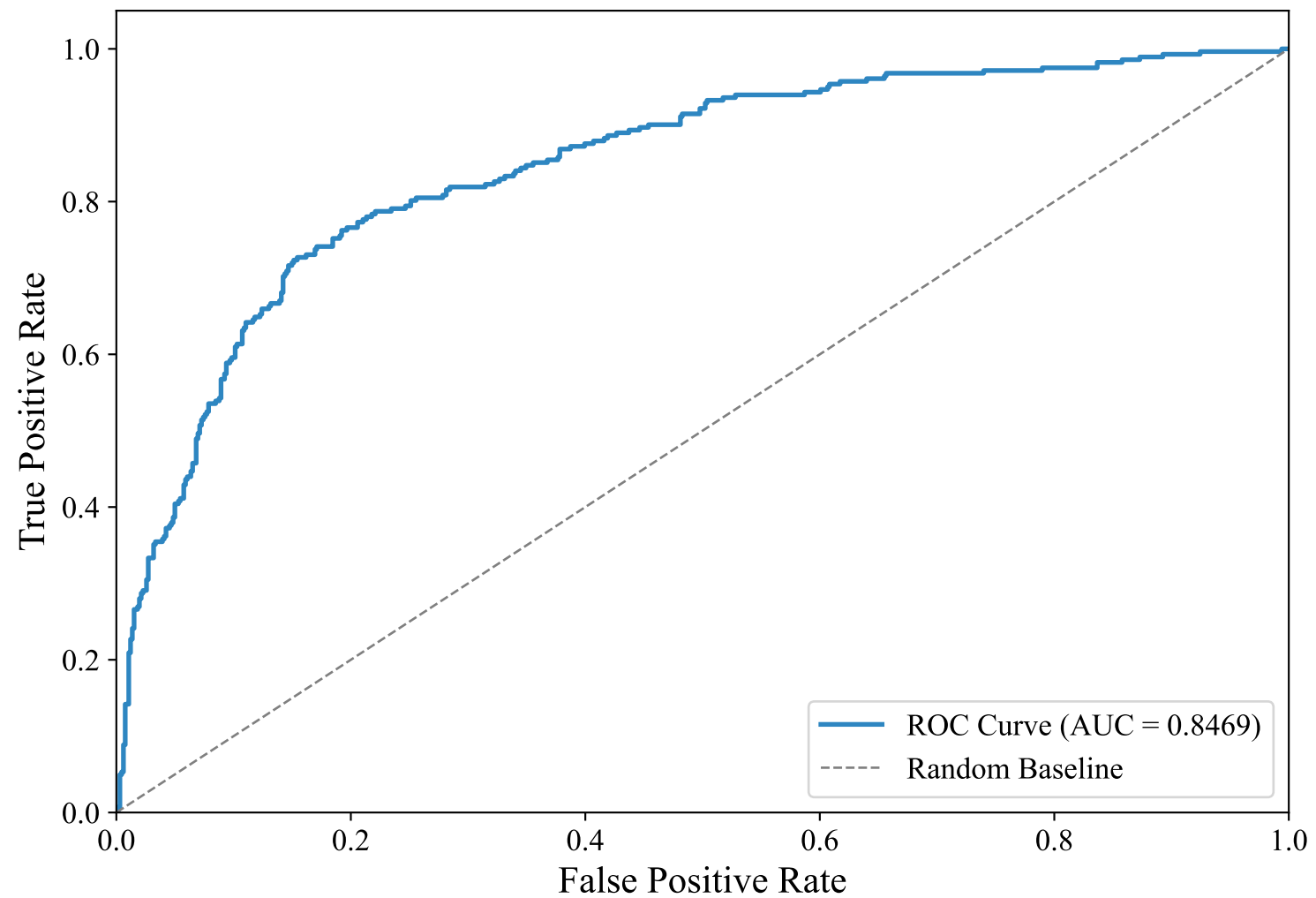
ROC Curve — ENGLISH_MANUAL (bert-base-multilingual-uncased, LightGBM_Optimized)
