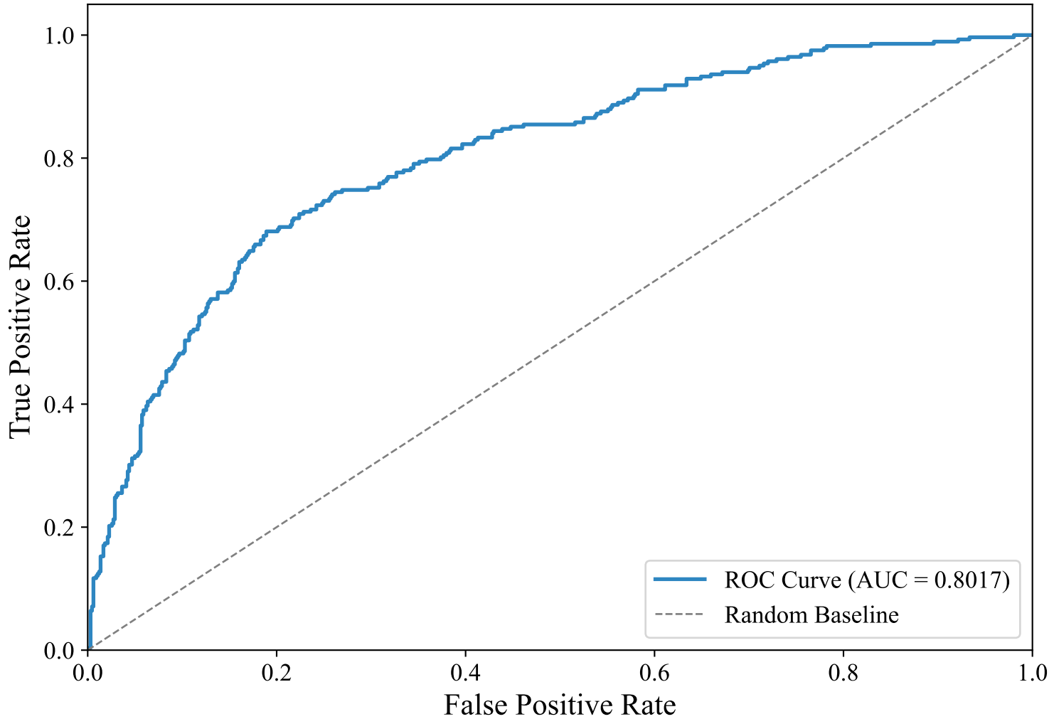
ROC Curve — ENGLISH_MANUAL (bert-base-multilingual-uncased, Random_Forest)
