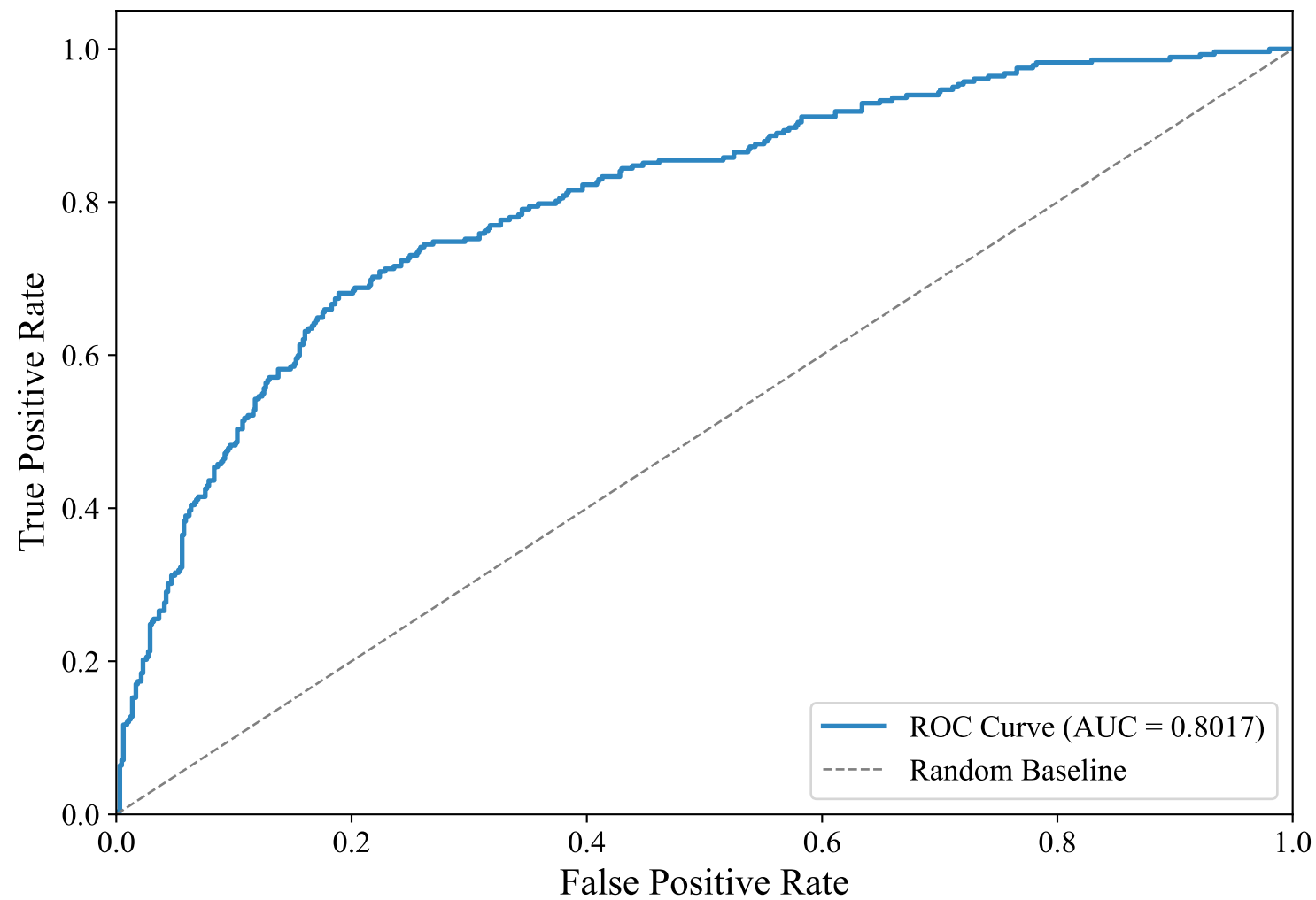
ROC Curve — ENGLISH_MANUAL (bert-base-multilingual-uncased, Random_Forest_Optimized)
