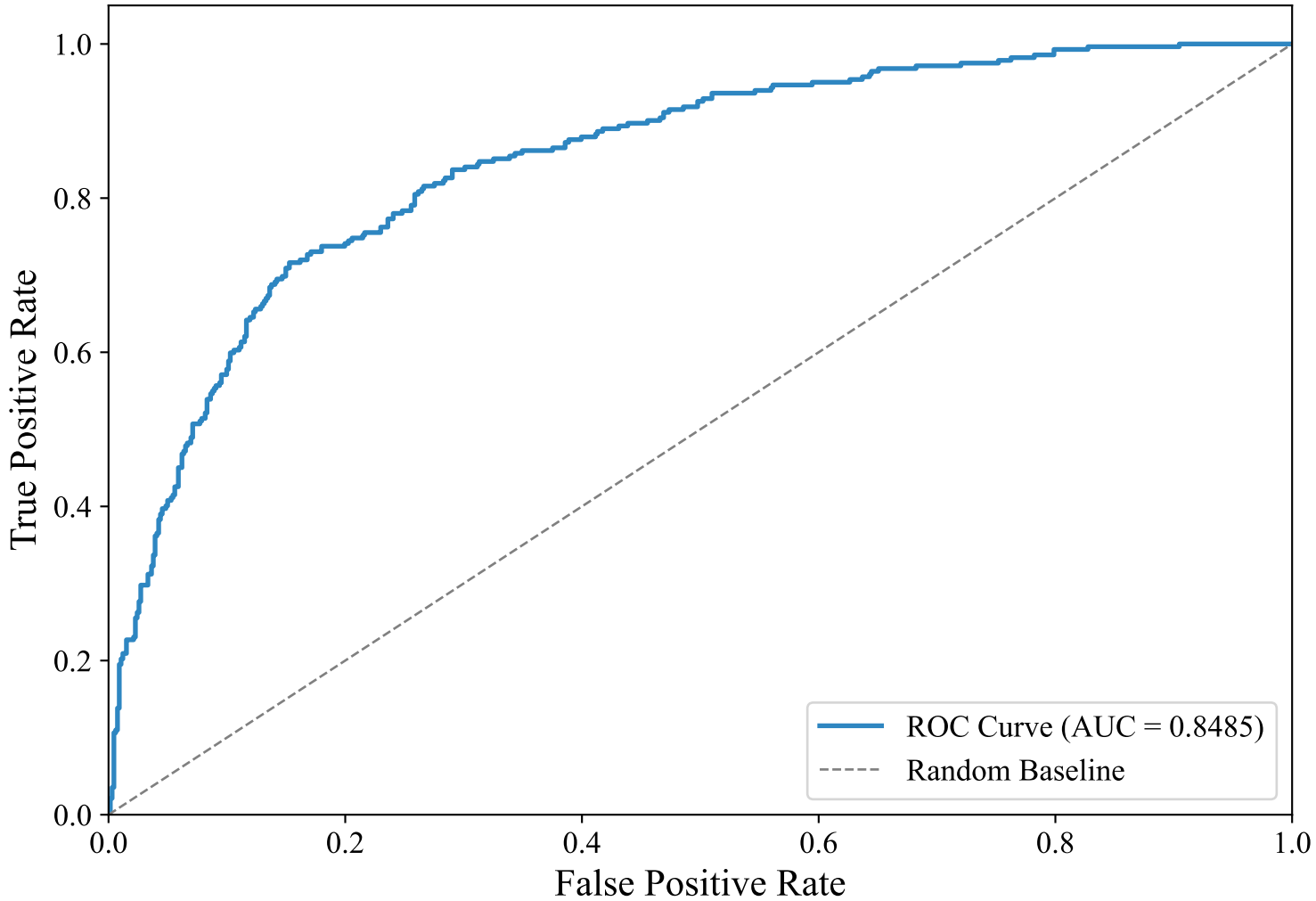
ROC Curve — ENGLISH_MANUAL (bert-base-multilingual-uncased, XGBoost)
