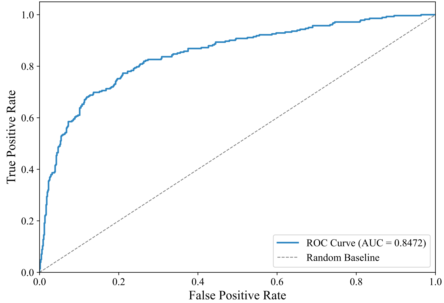
ROC Curve — ENGLISH_MANUAL (efederici/e5-base-multilingual-4096, LightGBM_Optimized)
