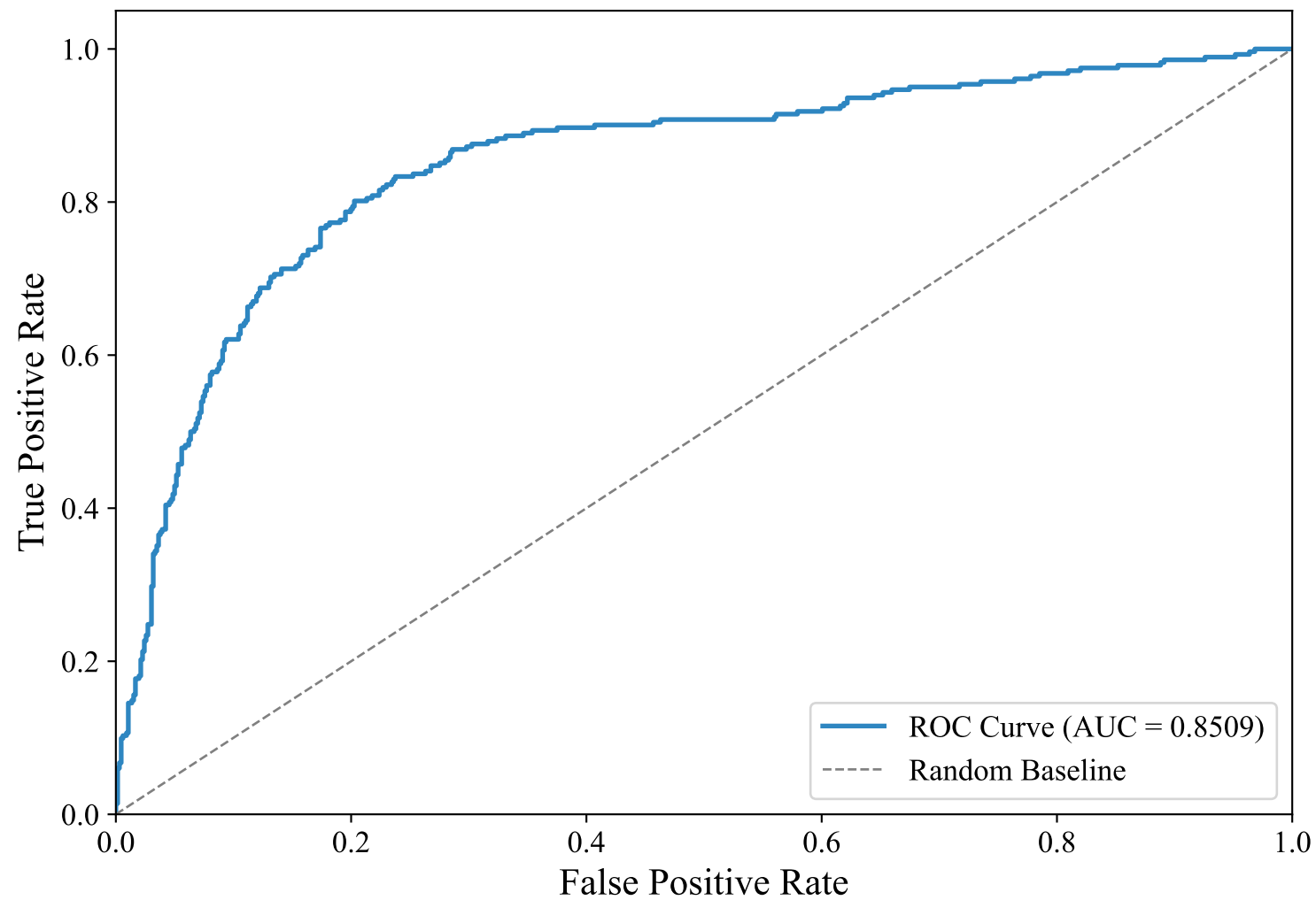
ROC Curve — ENGLISH_MANUAL (paraphrase-multilingual-MiniLM-L12-v2, Voting_Ensemble)
