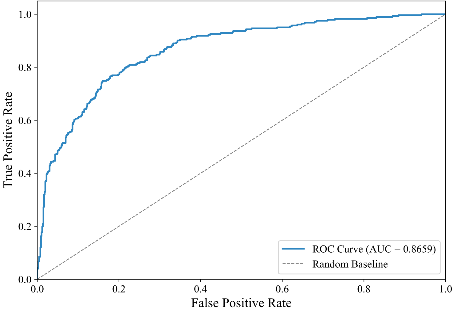
ROC Curve — ENGLISH_MANUAL (paraphrase-multilingual-mpnet-base-v2, LightGBM_Optimized)
